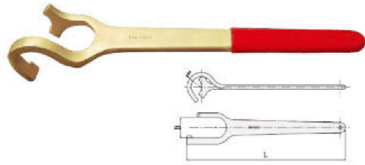
NS176C Valve Spanner
