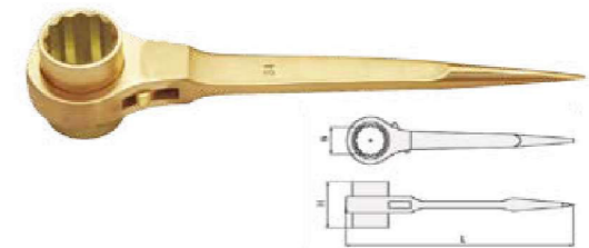
NS180 Ratchet Wrench
